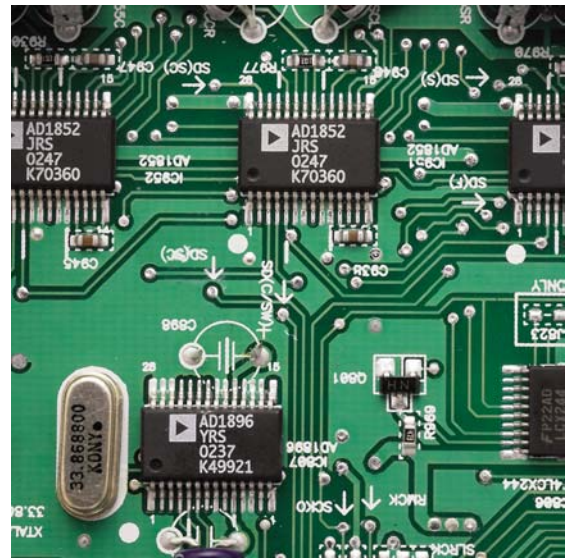
P-965, R-965 "Analog Devices" Chips Note: AD-1896 Digital Remastering Chip & AD-1852 24/192 Audio DAC's
