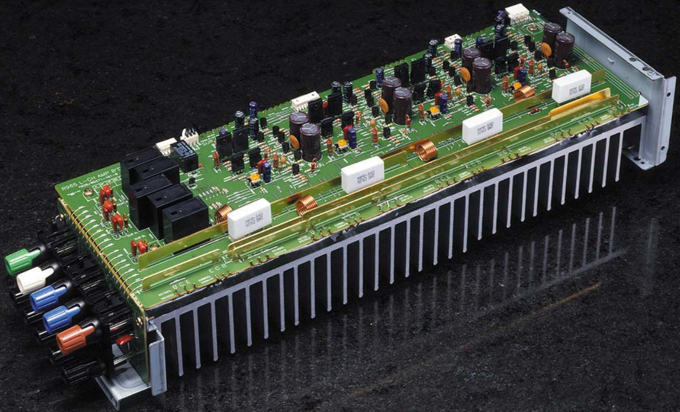
R-965 Center and Rear Amplifier Assembly. Note: Massive aluminum heatsinks, color coded binding posts, all discrete components.
